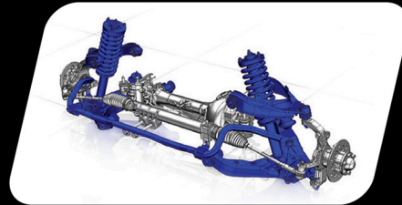
Front independent double wishbone suspension
